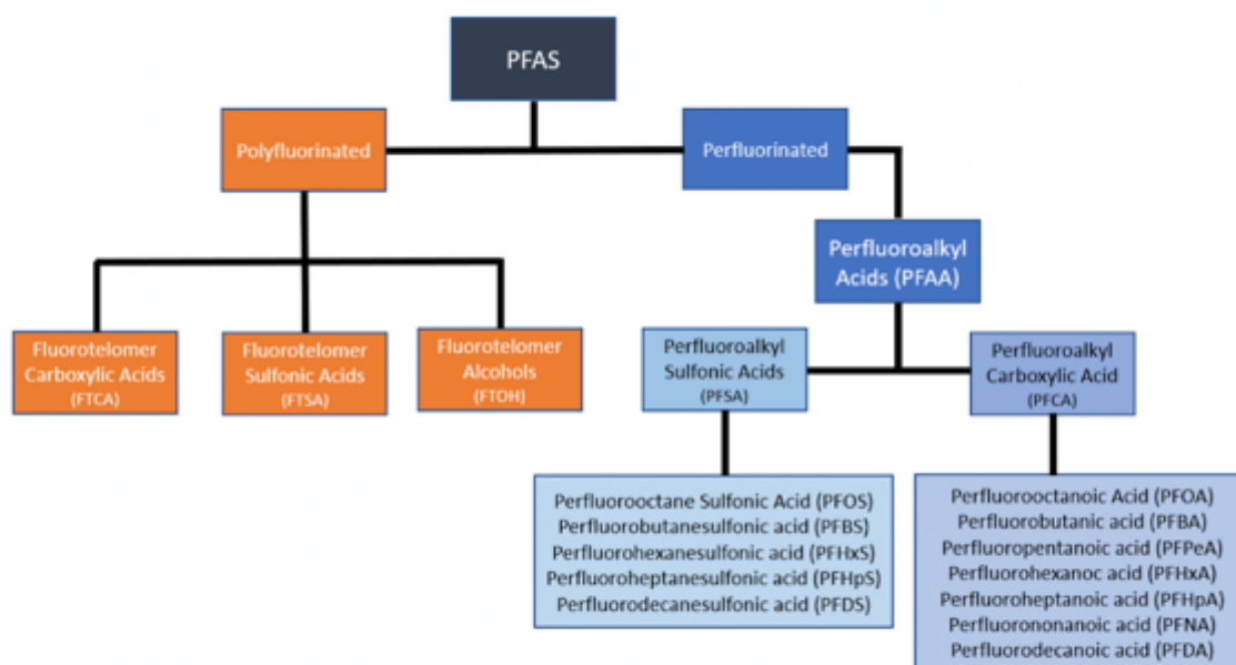
Figure 2: Basic family tree of PFAS
